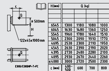
Triplex mast
