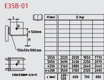
Standard, Duplex mast
