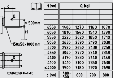
Triplex mast
