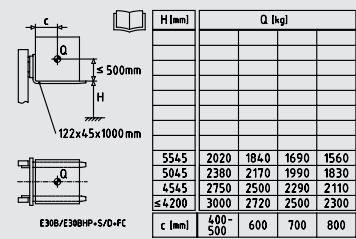
Standard, Duplex mast
